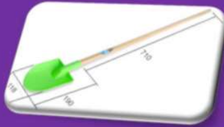
Article No. HH406-1 Kids Plastic Spade Varnished wood Handle Handle-710mm
